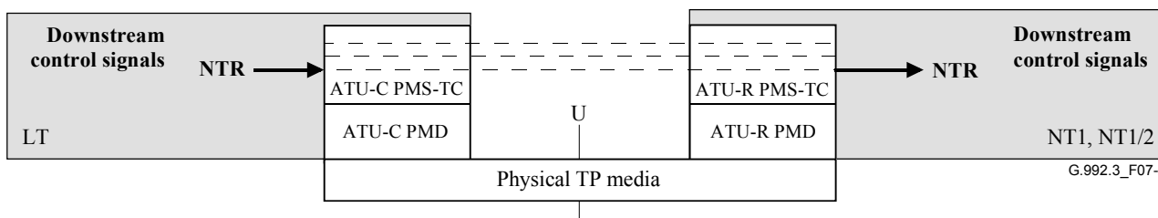
Figure 7-2/G.992.3 – PMS-TC transport capabilities within the control plane
